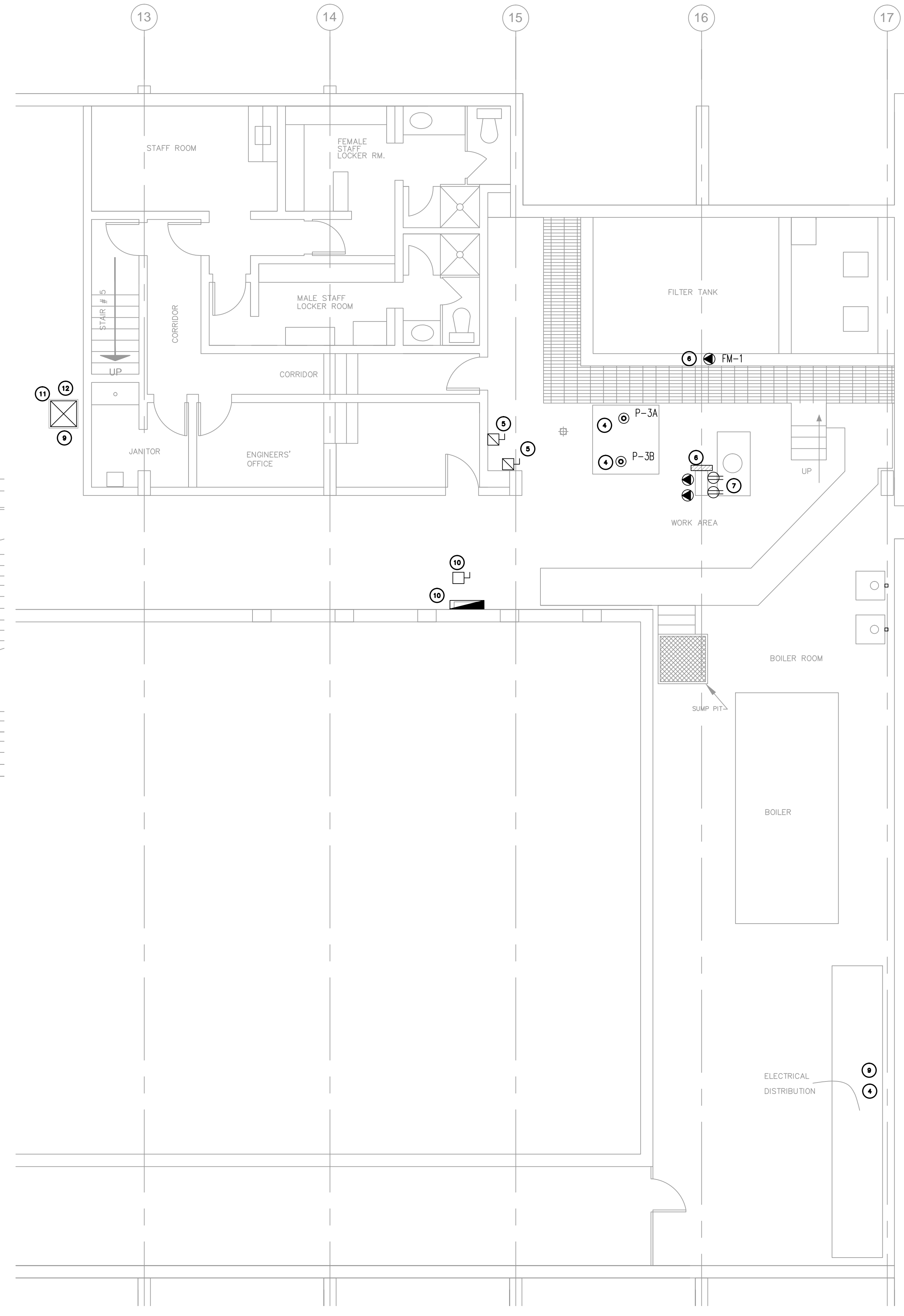
2 MECHANICAL ROOM PLAN - RENO E-1 SCALE: 3/16" = 1' - 0"
