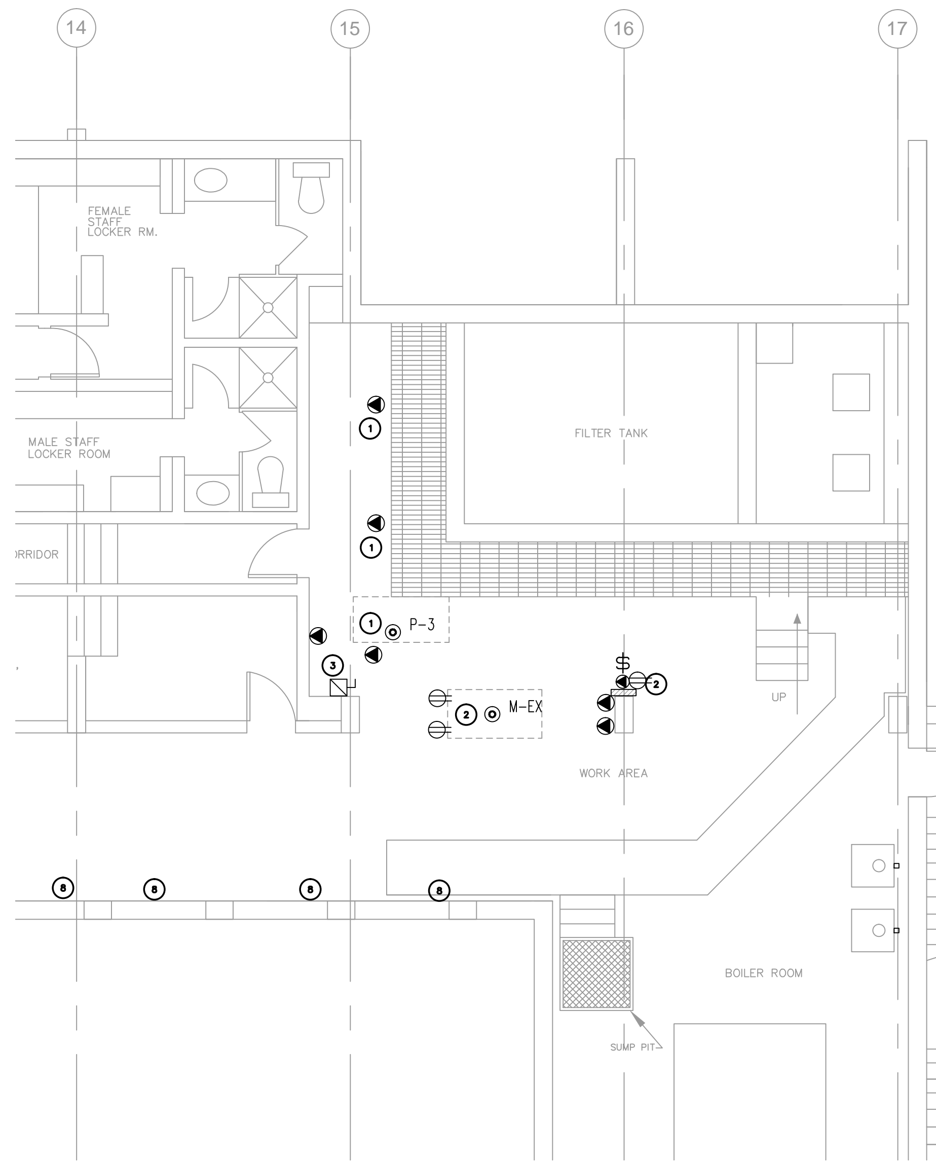
2 MECHANICAL ROOM PLAN - DEMO E-1 SCALE: 3/16" = 1' - 0"
